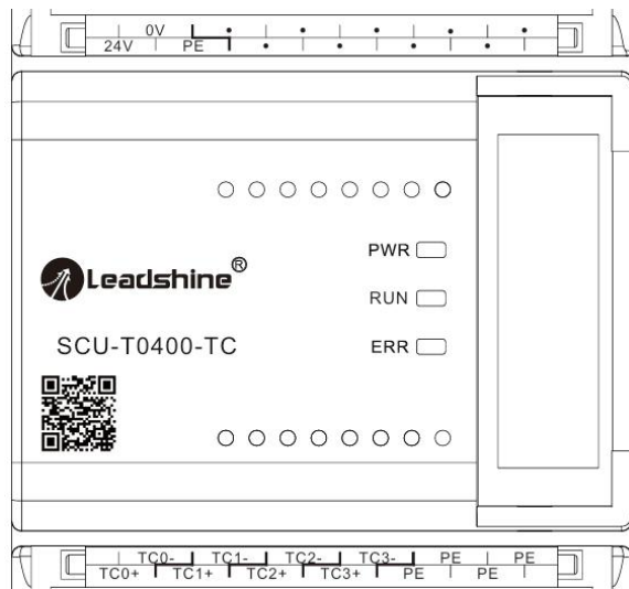
图 9-2 SCU- T0400-TC模块端子丝印
